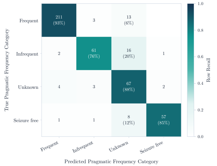
Fig. 6: Infrequent was the most error-prone category with 21% misclassified as unknown or seizure free.
