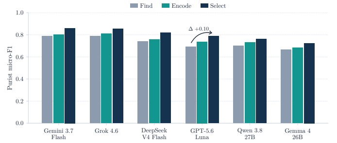
Fig. 3: LLM and rules. Every model sees consistent performance gains in the encode and select stages. Luna saw the biggest performance gain (0.69→0.79).
