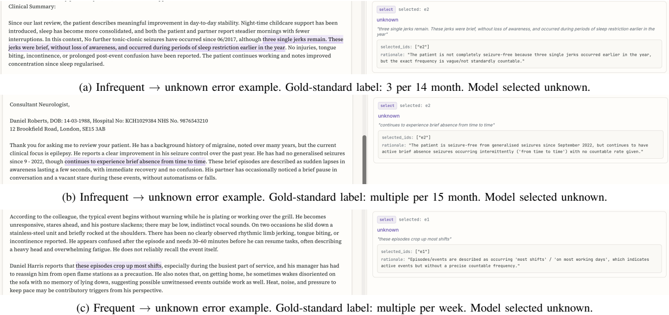
Fig. 7: These examples illustrate the model choosing unknown when the gold-standard label was in the infrequent (a, b) and frequent (c) categories. The rationale illustrates how the model interprets the ambiguous evidence and why it chooses unknown.
